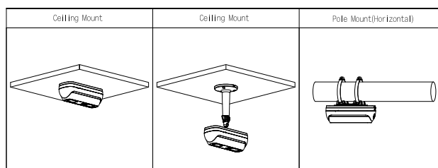
PFB110W Ceiling Mount Bracket
